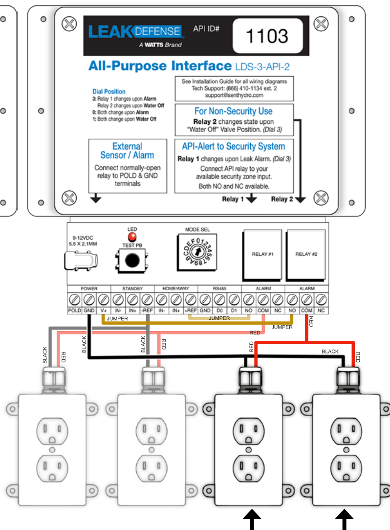
Alternate Wiring for 2 to 4 Recirc Pump Switches
